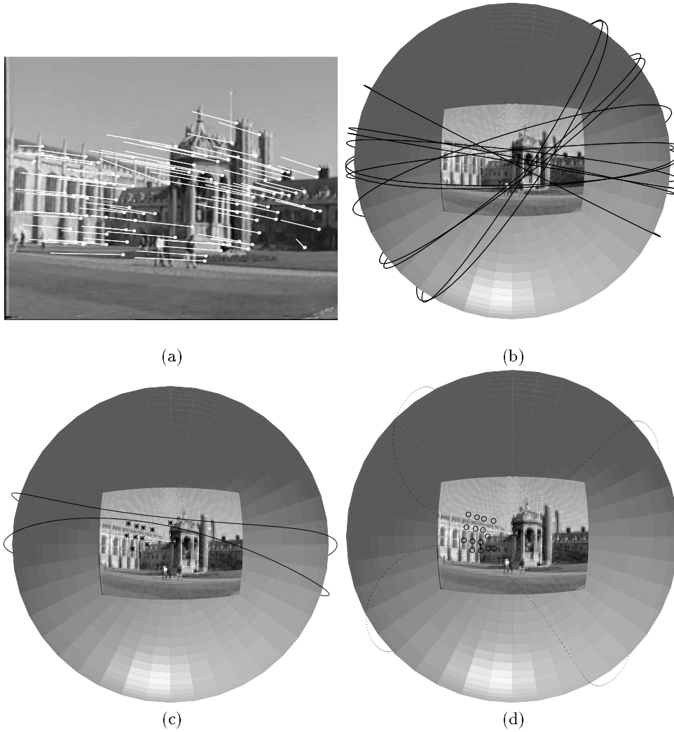
Fig.1. Subspace constraints and uncertainty estimates:: (a) shows the image feature displacements measured between two frames. The features were automatically extracted and matched and approximately 6 are incorrect correspondences. The translation of the camera was along the path just visible in the bottom right corner, but the image motion is mostly due to rotation. (b) shows the set of constraints obtained from 14 image regions by the Linearised Subspace Method. (c) shows the 95% uncertainty band and the image points contributing to the constraint. (d) shows an excessively uncertain constraint arising from distant points which are approximately on a plane
