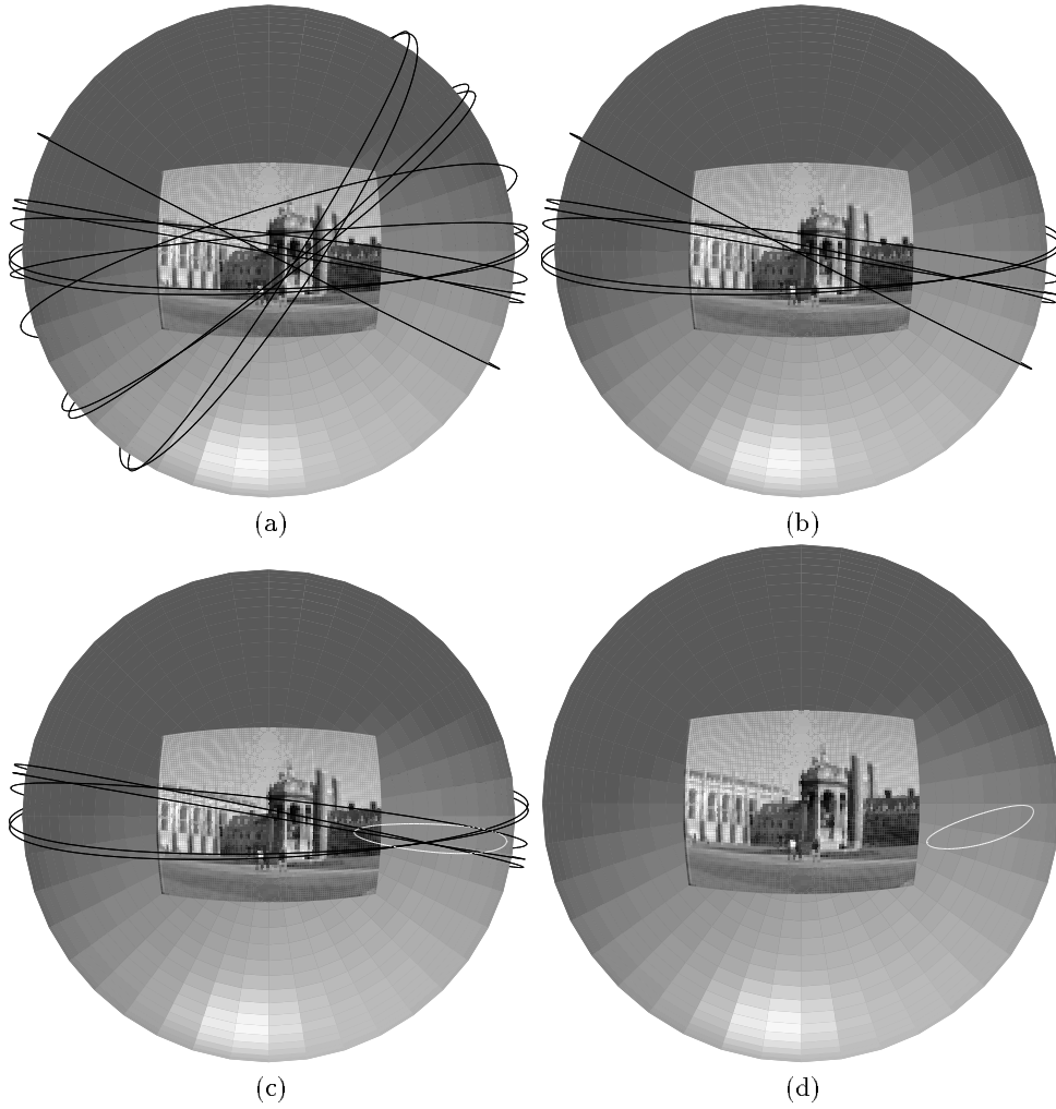
Fig. 3. The outlier rejection constraints: This figure gives a limited demonstration of the Consistency constraint and excessive error rejection for the features in Figure 1. (a) shows all the constraints found, (b) shows those with a reasonably small uncertainty and (c) shows all but one being accepted as agreeing with an epipole estimate, which is also shown as its 95% certainty ellipse. (d) shows the epipole ellipse given by the Fundamental Matrix calculated with the inliers and constrained to the epipole from (c).
