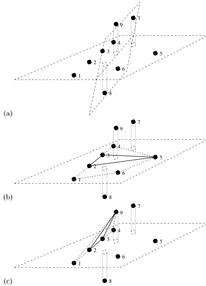
Fig.2. Example rejection problem: Because the rejection algorithms considered in this section are generally applicable, a low-dimensional example problem will be used to introduce them: find a plane that fits a large number of the 3D points in a set. Each picture above shows the six inliers (1-6), the three outliers (7-9), and the plane. (a) Poor initialisation using whole set: Outliers are often of greater magnitude than true measurements, and can therefore greatly influence any initialisation using the whole set (as shown). In this case, take-one-out cross-validation would also fail because we have three significant outliers. (b) Good solution from random initialisation set: If the assembling of the plane estimate is initialised by three correct points (eg. 2, 3 and 5 as shown) then the other points can also be found. An average of four random trials (approximately) will be needed to find the plane. (c) False solution from degenerate structure: Solutions can also appear to be found when the verification comes from degenerate structure. Points 1 and 4 appear to be verifying the plane found from 2, 3 and 9, because they form a degenerate structure (a line) with all but one of these points. This effect should not cause trouble when a good solution can be found, as it will receive better verification (as in (a)). However, when the scene is truly degenerate, this can cause an (often strong) false positive.
